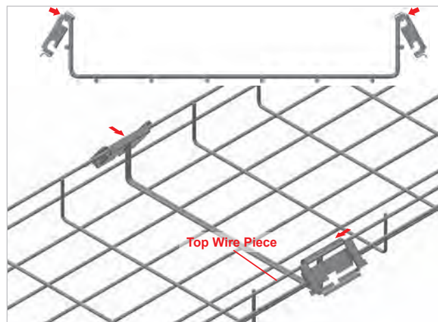
■ Upper wire slot of the lateral joint element is placed as angular on upper wire of wire mesh.
